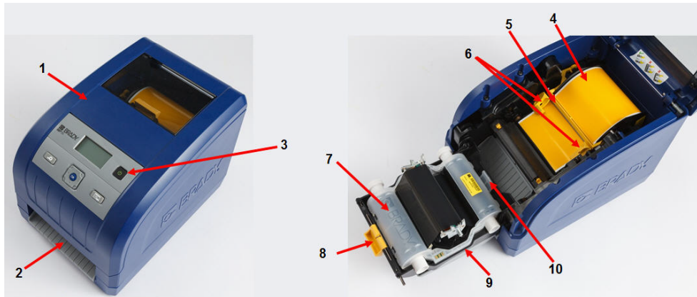
Figure 1 • Printer Components
